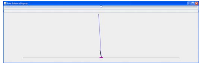
Fig. 2. Double pole balance simulator GUI display. The horizontal block represents the cart. The two vertical lines indicate the deflection the short and long pole, respectively. The line beneath the cart is the track. Letting a pole fall more than 36^\circ from vertical or running off the track constitutes failure. To prove itself to be a valid solution, an ANN must pass 10 trials, each lasting 100,000 simulation steps.
