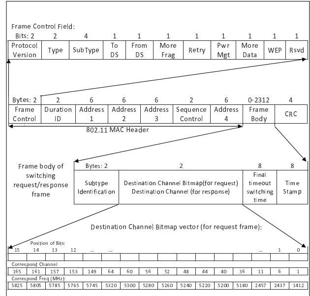
Fig. 2. Detail structure of switching request/response frame
