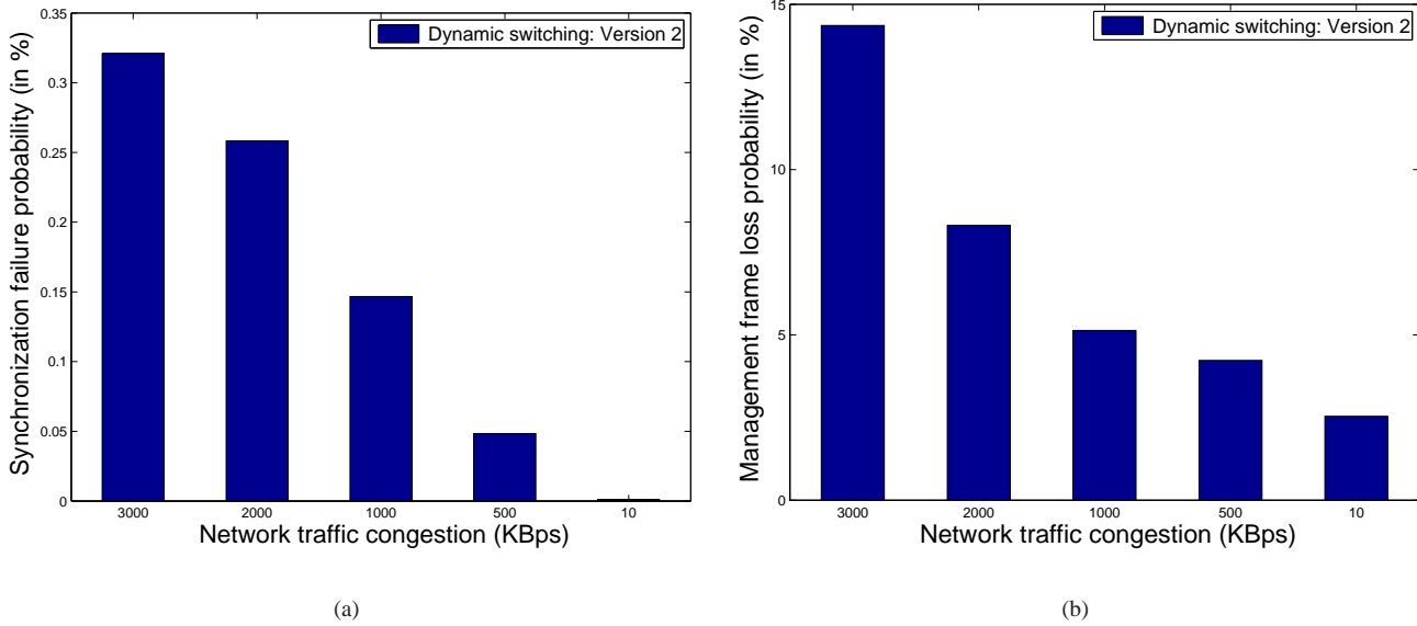
Fig. 4. a) Synchronization failure probability with version 2; b) Channel switching request frame loss probability with version 2
