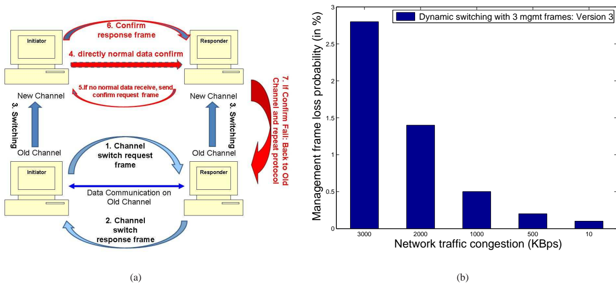
Fig. 5. a) Dynamic Frequency Switching: Version 3; b) channel switching request frame loss probability with version 3
