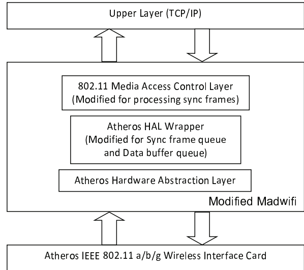
Fig. 1. Proposed protocol stack for SpiderRadio
