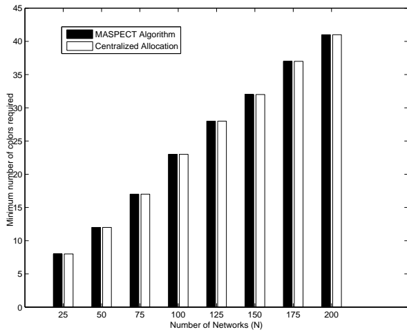
(a) Minimum number of colors required
