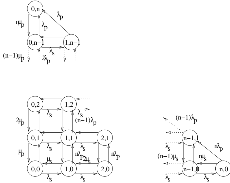
Fig. 4. CTMC that models the channel occupancy in a DSA network in the presence of primary activity.
