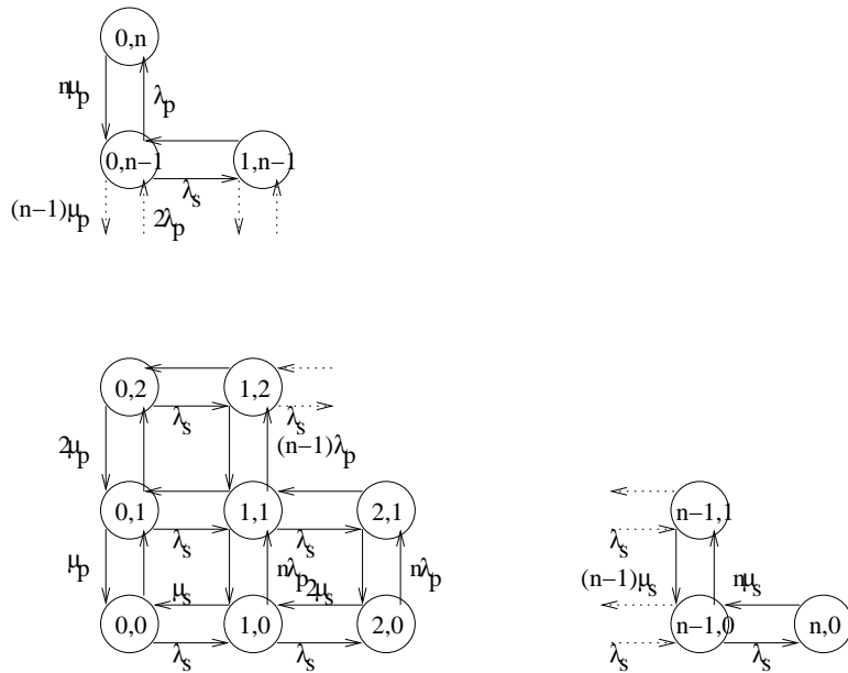
Fig. 5. Modified CTMC that approximately models the channel occupancy in a DSA network in the presence of primary activity. This is obtained by neglecting transitions from state (s, p) to (s - 1, p + 1) when s + p = n in Fig. 4.
