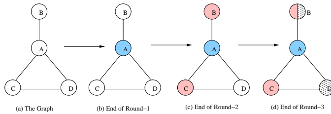
Fig. 2. Color assignment sequence when Steps 1-5 of the MASPECT Algorithm are applied to a sample graph.
