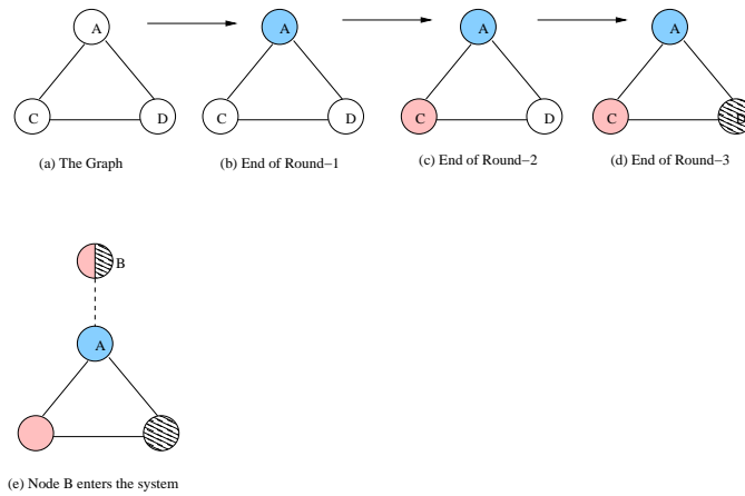
Fig. 3. Example to illustrate how Algorithm 1 adapts to the entry of a new node in the system. Color assignment sequence when Steps 1-5 of Algorithm 1 are applied to the graph in (a) are shown in (b) – (d). A new node (node B) then enters the system.
